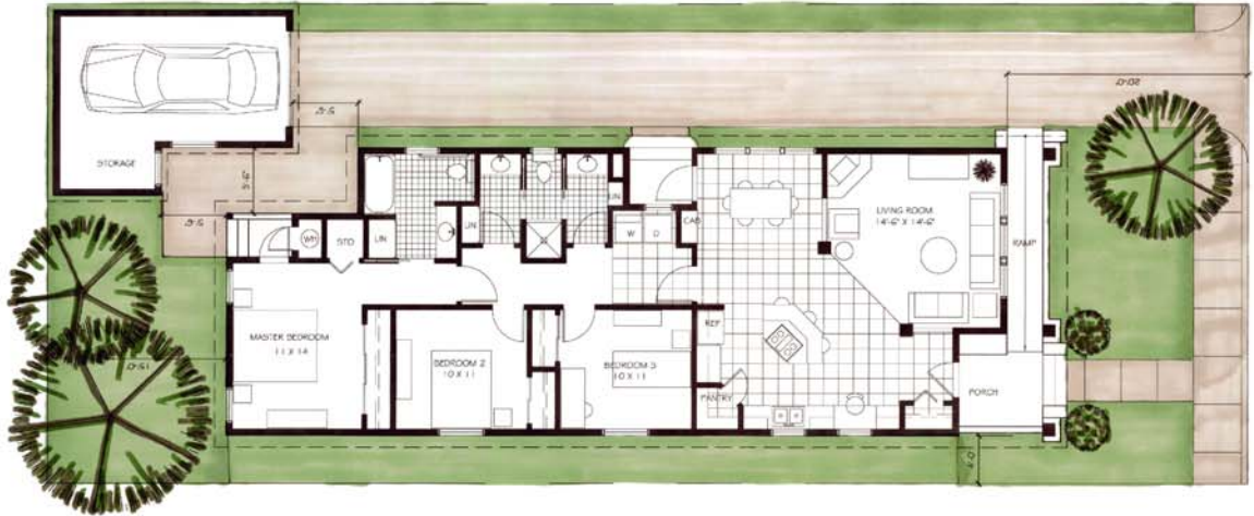
FLOOR PLAN - THREE BEDROOM / TWO BATH 1450 SQUARE FEET
